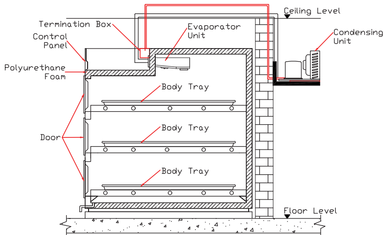
Side View Model : 3301-RA (Remote Type Compressor)
