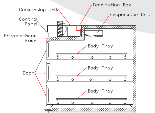
Side View Model : 3301-FA (Front Compressor)
