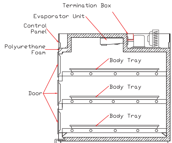
Side View Model : 3301-BA (Back Compressor)
